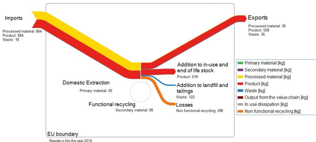
Figure 23. Simplified Sankey diagram for scandium for the year 2016 in the EU (without the UK). Imports of processed material include 792 kg Sc in scandium compounds and 72 kg Sc in Sc-Al master alloys or scandium metal, respectively. Imports of products include 255 kg Sc of Al-Sc alloys, SOFCs and airplanes containing Sc.
