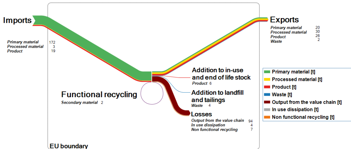
Figure 9. Simplified Sankey diagram for hafnium for the year 2016 in the EU (without the UK).
