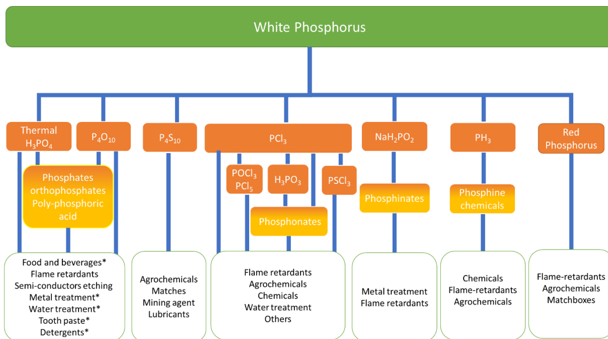
Figure 19. Simplified chemical family of P_4 , derivatives, intermediates, products and final applications * applications that can be obtained from thermal phosphoric acid or purified wet phosphoric acid.
